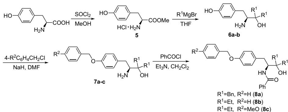
Scheme 1. Synthesis of chiral ligands 8a–c .
